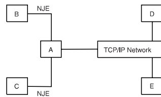
Figure 15. SMTP as a mail gateway
